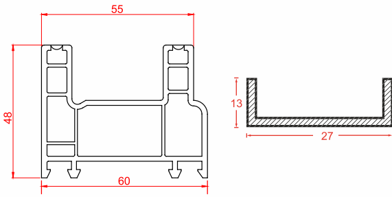
Name: Two Track (50) | Code: SWH50-01 Weight: 0.93 kg/m Pkt Qty: 6 pcs
