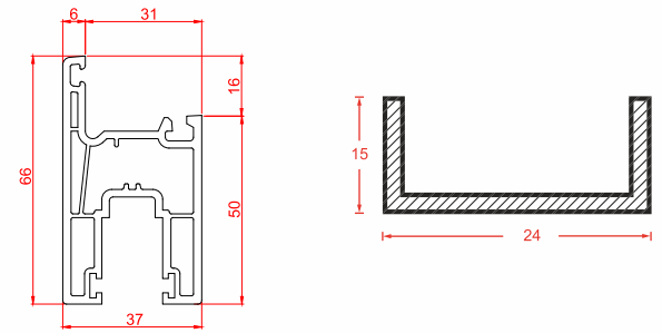
Name: Sliding Super Sash 66mm | Code: SWH50-04 Weight: 0.98 kg/m Pkt Qty: 6 pcs
