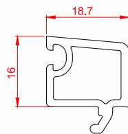
Name: Sliding 12mm Beading Code: SWH60-14 Weight: 0.23 kg/m Pkt Qty: 25 pcs
