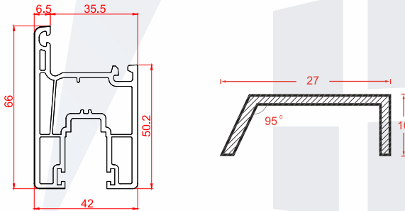
Name: Sliding Super Sash 66mm | Code: SWH60-04 Weight: 1.03 kg/m Pkt Qty: 6 pcs
