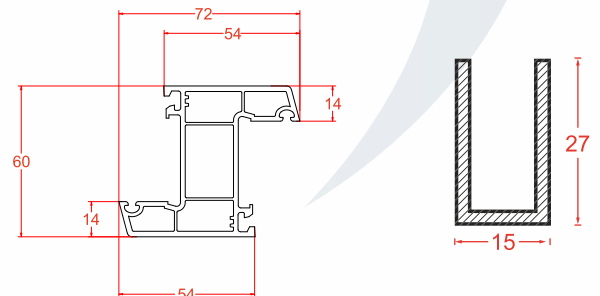
Name: Z Mullion | Code: CWH60-11 Weight: 1.06 kg/m Pkt Qty: 6 pcs
