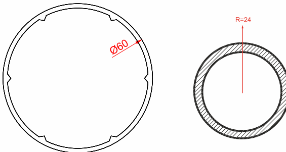
Name: Bay Pole | Code: AWH60-04 Weight: 0.50 kg/m | Pkt Qty: 7 pcs
