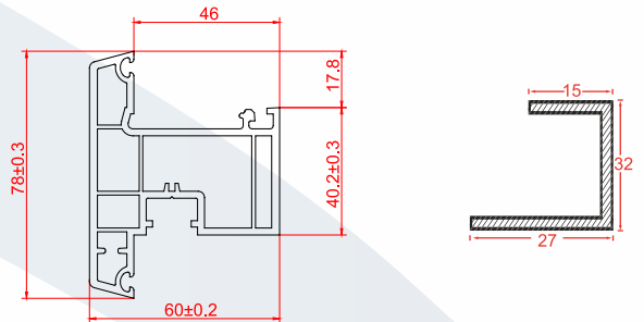
Name: Outward Window Sash | Code: CWH60-03 Weight: 1.21 kg/m Pkt Qty: 4 pcs
