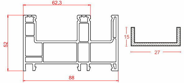
Name: 2.5 Track | SWH60-16 Weight: 1.36 kg/m Pkt Qty: 4 pcs
