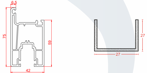
Name: Sliding Door Sash 75mm | Code: SWH60-05 Weight: 1.11 kg/m Pkt Qty: 6 pcs
