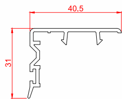
Name: Sliding Super Sash Intelock | Code: SWH50-07 Weight: 0.23 kg/m Pkt Qty: 25 pcs
