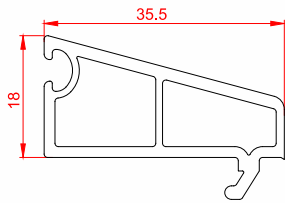
Name: Casement 6 mm Beading | Code: CWH60-08 Weight: 0.32 kg/m Pkt Qty: 25 pcs
