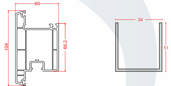
Name: Outward Door Sash | Code: CWH60-06 Weight: 1.51 kg/m Pkt Qty: 4 pcs
