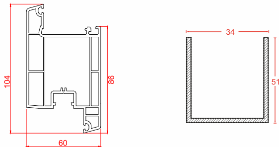
Name: Inward Door Sash | Code: CWH60-07 Weight: 1.54 kg/m Pkt Qty: 4 pcs
