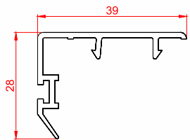
Name: Sliding Sash Interlock (50) | Code: SWH50-06 Weight: 0.20 kg/m Pkt Qty: 25 pcs
