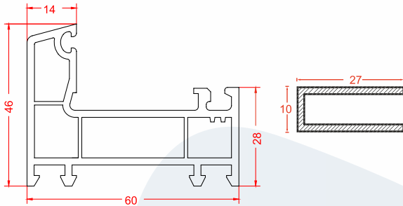
Name: Casement Frame 28mm | Code: CWH60-01 Weight: 0.87 kg/m Pkt Qty: 4 pcs
