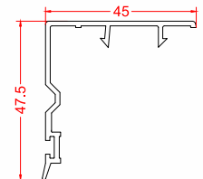
Name: Sliding Mega Sash Interlock Code: SWH60-11 Weight: 0.28 kg/m Pkt Qty: 25 pcs
