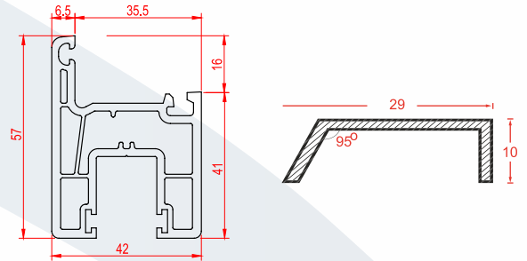
Name: Sliding Sash 57mm | Code: SWH60-03 Weight: 0.90 kg/m Pkt Qty: 8 pcs
