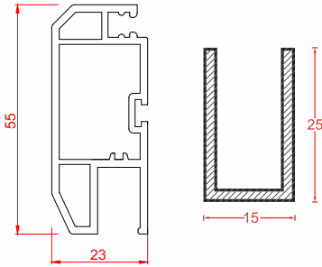
Name: Fly Mesh Sash | Code: SWH60-17 Weight: 0.48 kg/m Pkt Qty: 12 pcs
