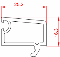
Name: Sliding 6mm Beading Code: SWH60-12 Weight: 0.26 kg/m Pkt Qty: 25 pcs
