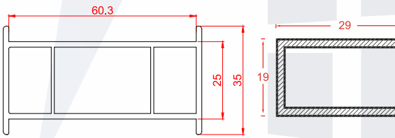
Name: Heavy Duty Coupling | Code: AWH60-06 Weight: 0.53 kg/m | Pkt Qty: 6 pcs
