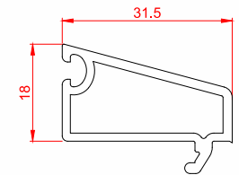
Name: Sliding Mesh Beading Code: SWH60-15 Weight: 0.28 kg/m Pkt Qty: 20 pcs
