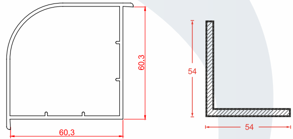
Name: 90 Degree Coupling | Code: AWH60-02 Weight: 0.65 kg/m | Pkt Qty: 4 pcs
