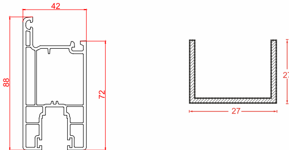
Name: Sliding Mega Sash 88mm | Code: SWH60-06 Weight: 1.25 kg/m Pkt Qty: 4 pcs
