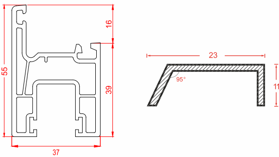
Name: Sliding Sash 55mm | Code: SWH50-03 Weight: 0.73 kg/m Pkt Qty: 8 pcs
