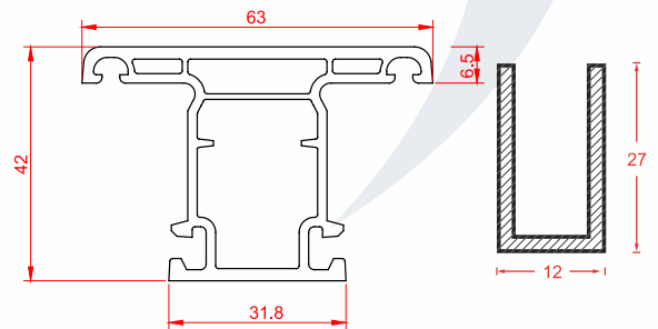
Name: Sliding Mullion | Code: SWH60-07 Weight: 0.80 kg/m Pkt Qty: 8 pcs
