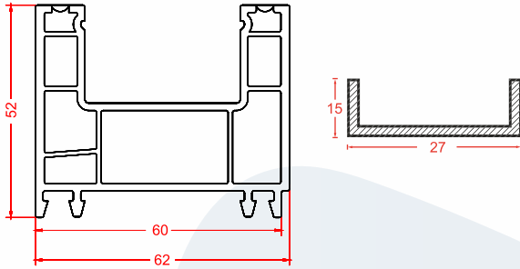
Name: Two Track | Code: SWH60-01 Weight: 1.02 kg/m Pkt Qty: 6 pcs
