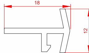
Name: T Joint Coupling | Code: AWH60-07 Weight: 0.08 kg/m | Pkt Qty: 50 pcs
