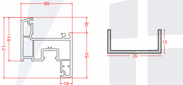
Name: Inward Window Sash | Code: CWH60-04 Weight: 1.15 kg/m Pkt Qty: 6 pcs
