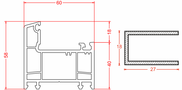
Name: Casement Frame | Code: CWH60-02 Weight: 1.05 kg/m Pkt Qty: 4 pcs
