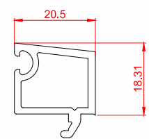
Name: Sliding 6mm Beading | Code: SWH50-05 Weight: 0.25 kg/m Pkt Qty: 25 pcs
