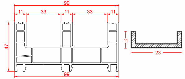
Name: Three Track (50) | Code: SWH50-02 Weight: 1.35 kg/m Pkt Qty: 4 pcs
