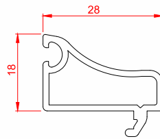
Name: Casement 12 mm Beading | Code: CWH60-09 Weight: 0.24 kg/m Pkt Qty: 30 pcs
