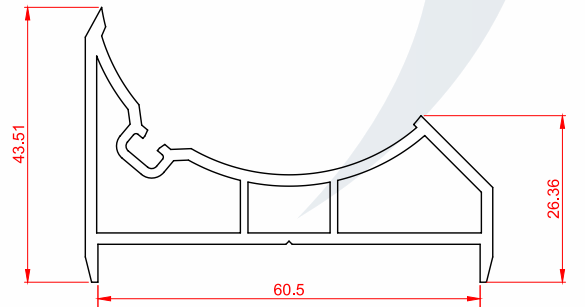
Name: Bay Pole Adaptor | Code: AWH60-05 Weight: 0.50 kg/m | Pkt Qty: 8 pcs
