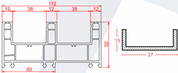
Name: Three Track | Code: SWH60-02 Weight: 1.71 kg/m Pkt Qty: 4 pcs
