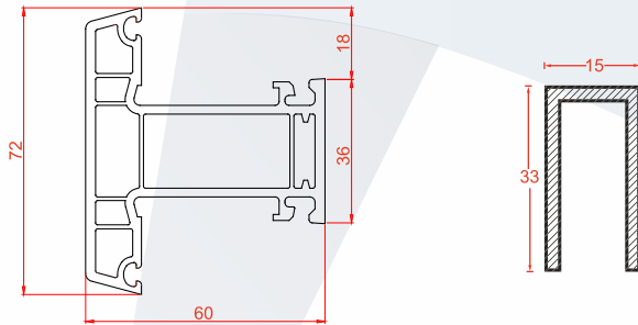
Name: Casement Mullion | Code: CWH60-05 Weight: 1.15 kg/m Pkt Qty: 6 pcs
