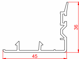
Name: Sliding Super Sash Interlock Code: SWH60-09 Weight: 0.24 kg/m Pkt Qty: 25 pcs
