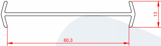
Name: Mini Coupling | Code: AWH60-01 Weight: 0.20 kg/m | Pkt Qty: 20 pcs
