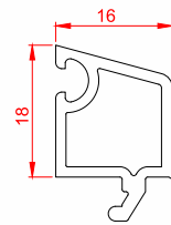
Name: Casement 24 mm Beading | Code: CWH60-10 Weight: 0.19 kg/m Pkt Qty: 40 pcs
