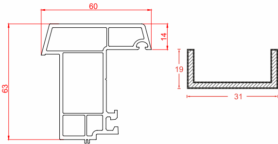
Name: Fly Mullion | Code: CWH60-12 Weight: 0.85 kg/m Pkt Qty: 6 pcs
