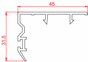
Name: Sliding Sash Interlock Code: SWH60-08 Weight: 0.23 kg/m Pkt Qty: 25 pcs
