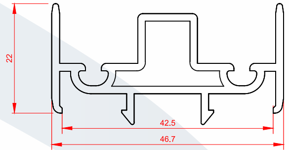
Name: Infill Sash Panel | Code: AWH60-09 Weight: 0.39 kg/m | Pkt Qty: 20 pcs
